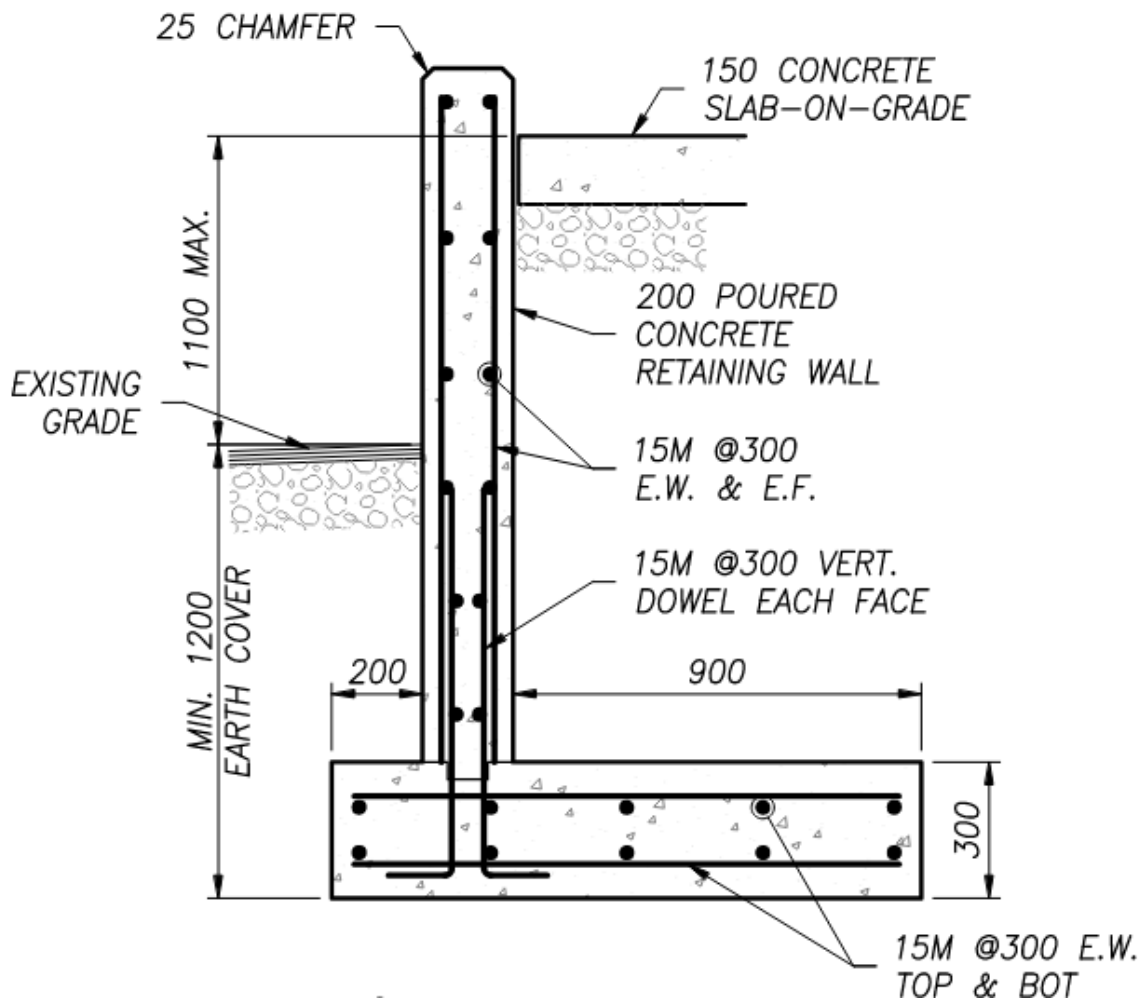
SECTION AT RETAINING WALL
